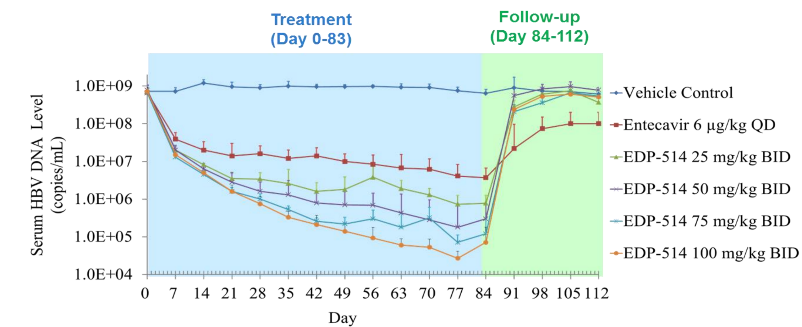
Figure 5. HBV DNA level over time
