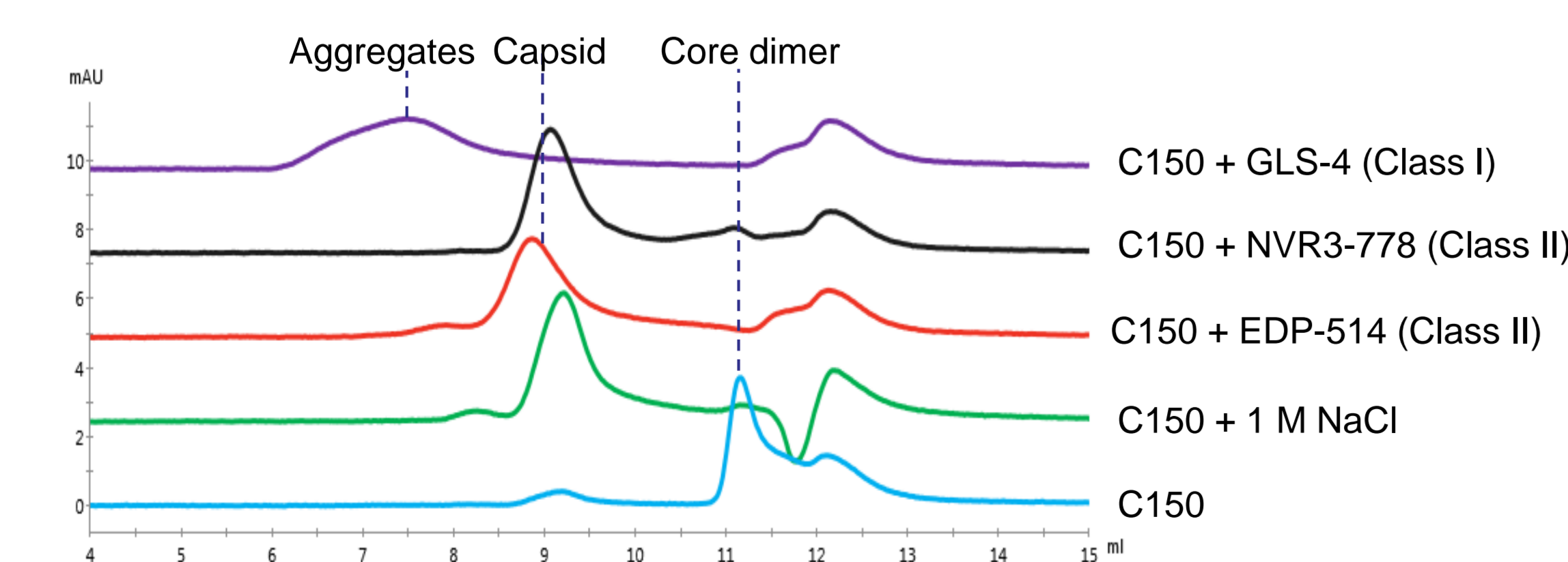
Figure 3. Size exclusion chromatography (SEC) analysis of capsid formation. Dimeric HBV core protein (C150) (2 µM) was incubated with either 1 M NaCl or 25 µM compounds 2 h and then analyzed using a SRT SEC 1000 column (14.29 mL). MW=16.78 kDa (C150); 33.56 kDa (dimer) 4000 kDa (capsid).
