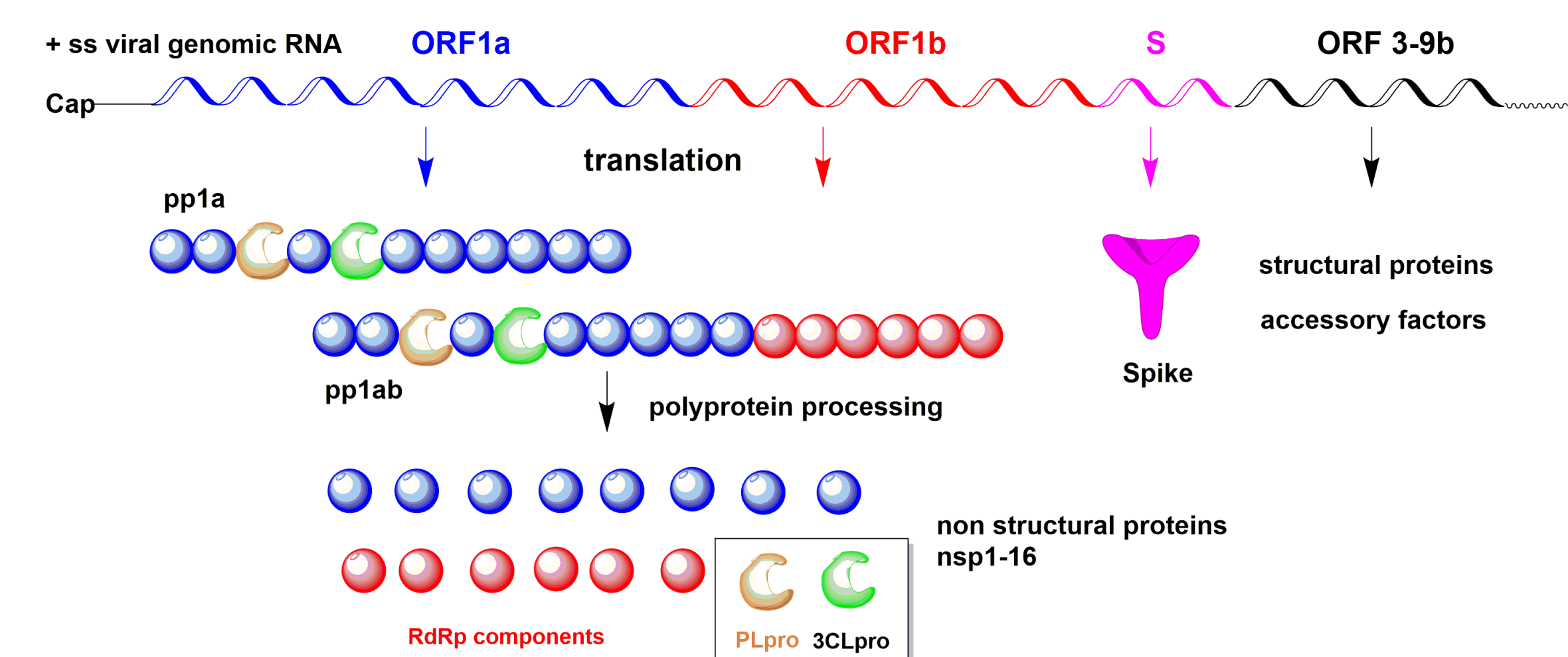
Figure 1. Role of 3CLpro in SARS-CoV-2 viral replication
