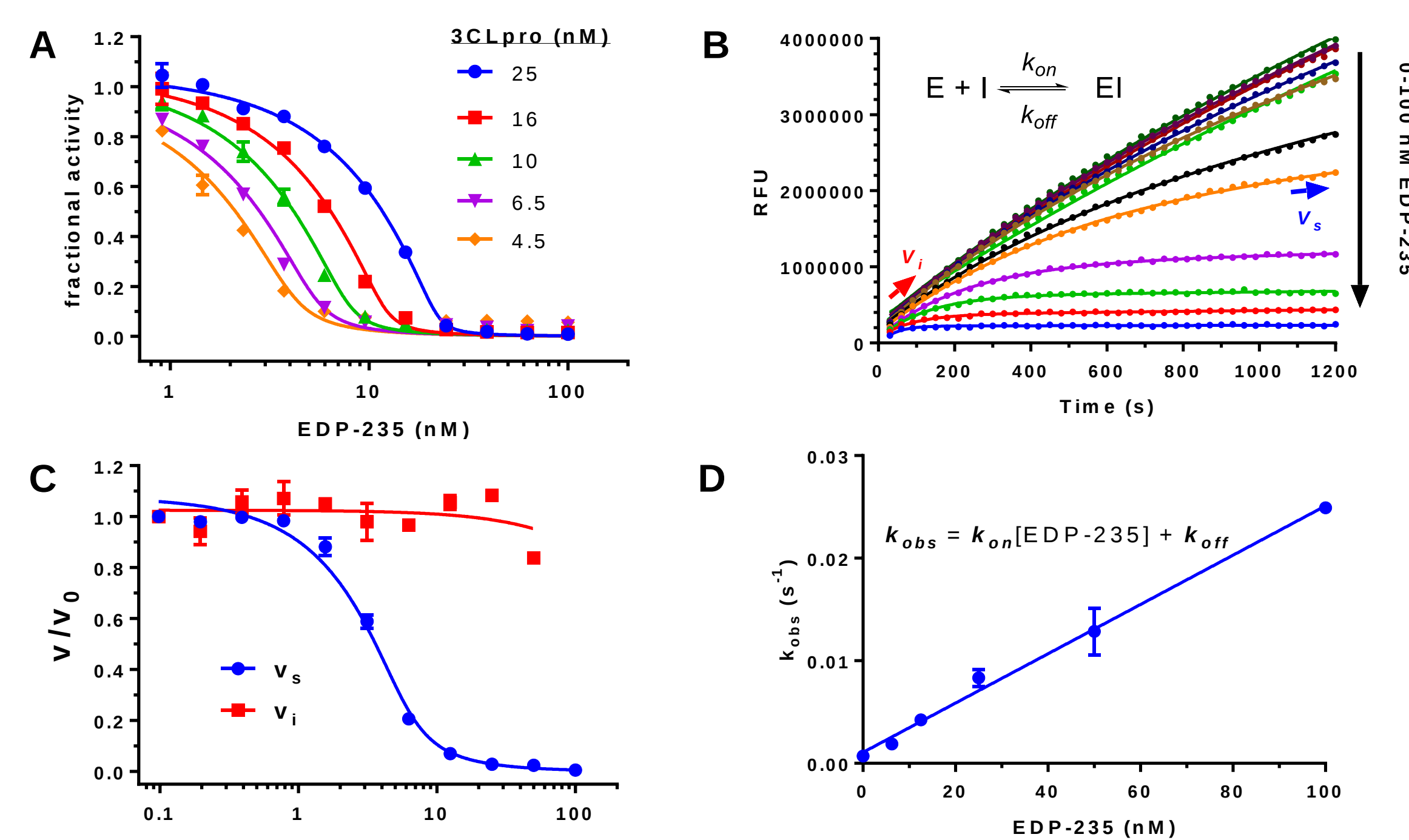
Figure 3. Kinetics of SARS-CoV-2 3CLpro inhibition by EDP-235.
