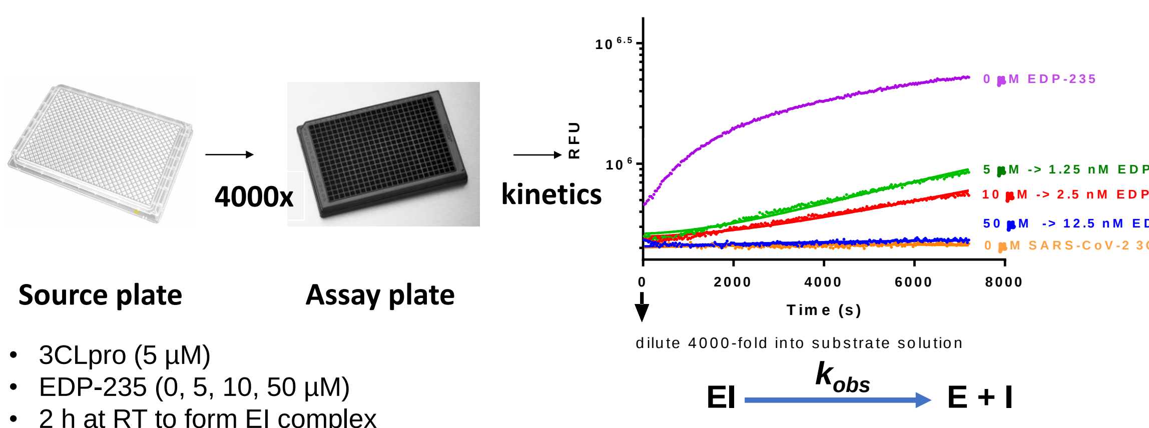
Figure 4. Jump dilution reversibility test for 3CLpro inhibition by EDP-235. (A) Jump dilution experimental setup and conditions. (B) Progress curves of 3CLpro activity after 4000-fold dilution into substrate solution. Representative data are mean of triplicate curves (N=3)
