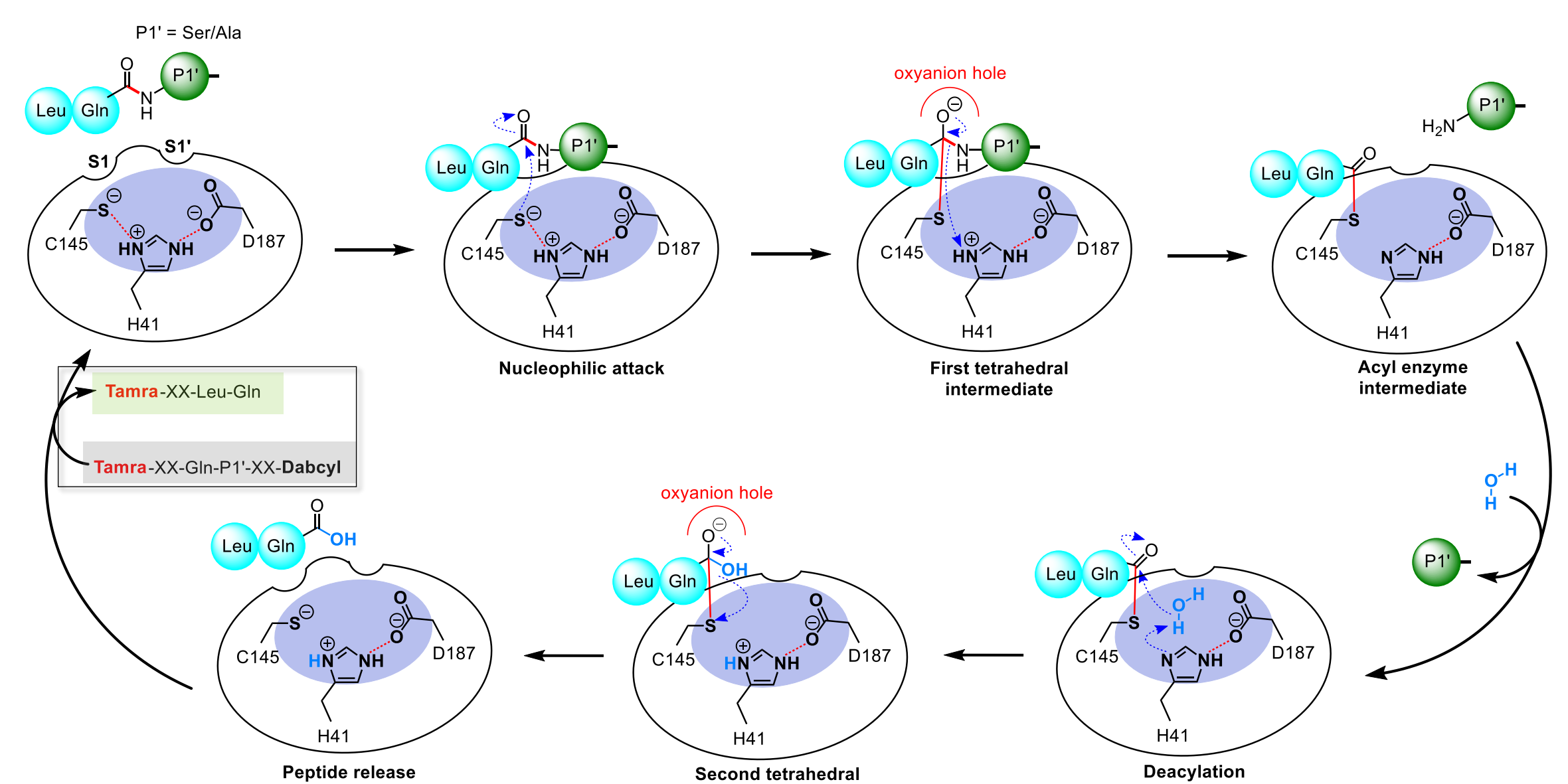
Figure 2. Catalytic mechanism of SARS-CoV-2 3CLprotease
